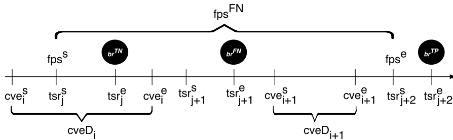
Figure 6-15 False negative failed-passed-sequence ( fps^{FN} ) with true negative and false negative basic test result ( br^{TN} & br^{FN} )
