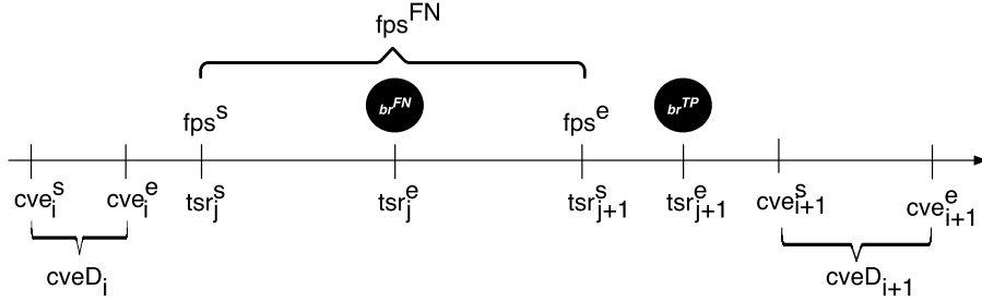
Figure 6-14 False negative fps
