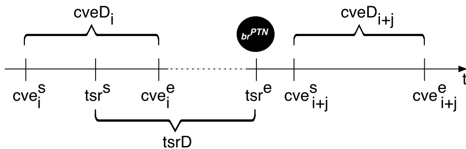
Figure 6-12 Pseudo true positive basic test result ( br^{PTN} )
