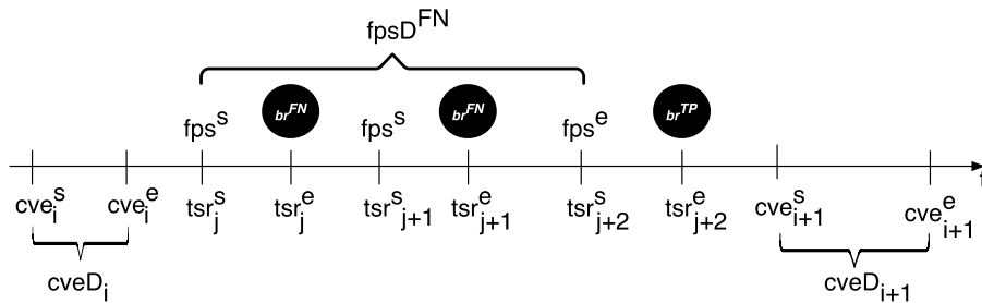
Figure 6-21 False negative Failed-Passed-Sequence-Duration ( fpsD^{FN} )
