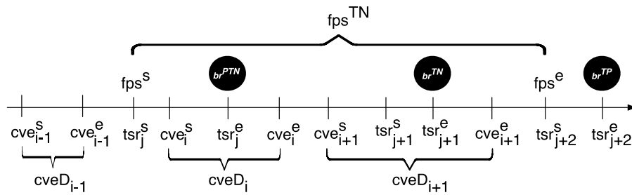
Figure 6-13 True negative failed-passed-sequence ( fps^{TN} )
